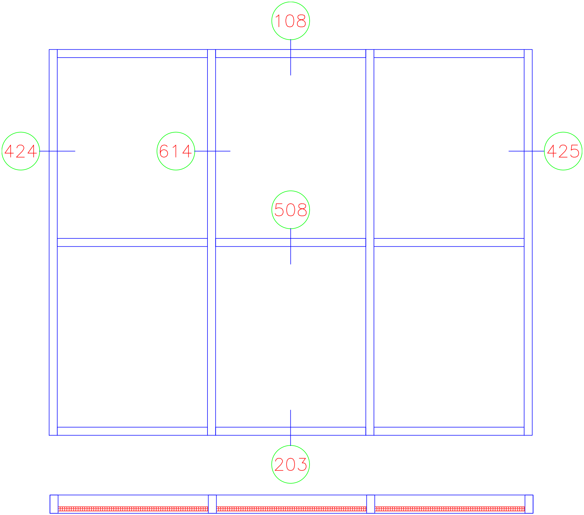
S433 Outside Glazed Outside Set 2" x 4 1/2" Screw Spline
